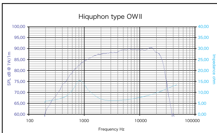
Frequency curve
